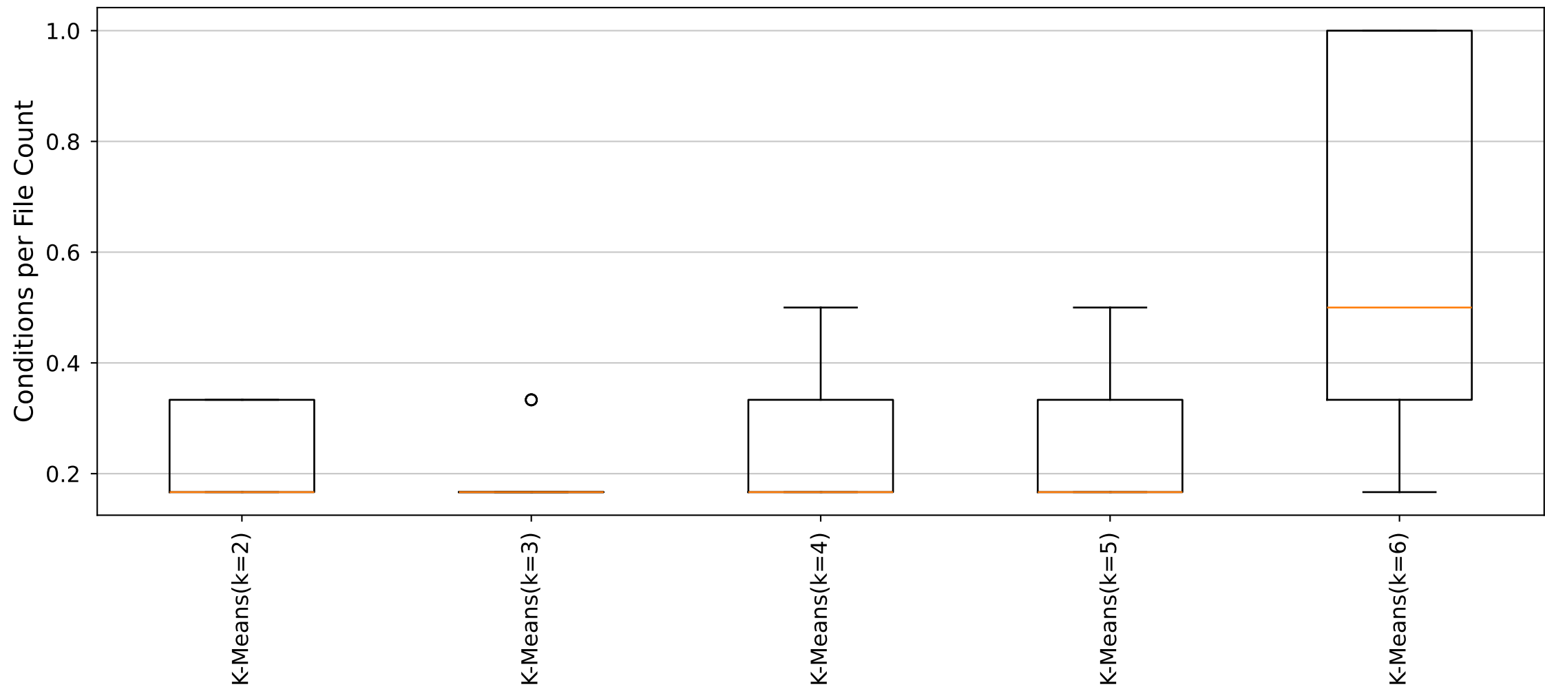
YARA Rules Conditions per File Count Distribution (Cluster29_Size6 dataset)
